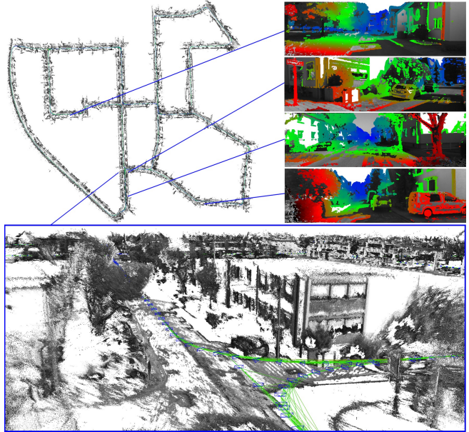
Fig. 1. Stereo LSD-SLAM is a fully direct SLAM method for stereo cameras. It runs at 30Hz on a CPU, computing accurate camera movement as well as semi-dense probabilistic depth maps. We exploit both static and temporal stereo and correct for affine lighting changes, making the method both accurate and robust in real-world scenarios. Some examples are shown in the attached video.
