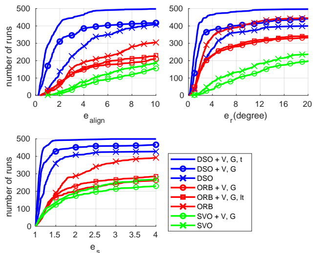
Fig. 3: Performance comparison of DSO, ORB-SLAM and SVO on sequences with/without photometric calibration (camera response function G , vignetting factors V ). The alignment error e_{align} , rotation drift e_r (in degree) and scale drift e_s are shown in the corresponding subplots. "It" stands for loosed thresholds for ORB feature extraction. For reference, we also show results of DSO using camera exposure times t .
