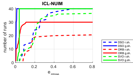
(a) Performances of the selected methods.
