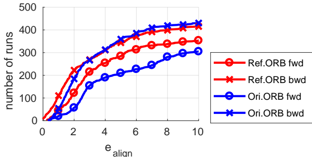
Fig. 10: Performance comparison between the original ORB-SLAM and our refined version on the full TUM Mono VO Dataset. With sub-pixel accuracy refinement of feature matching, ORB-SLAM performs better running forward and similarly running backward.
