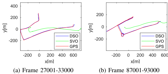
Fig. 12: Estimated trajectories of the segments of the Frankfurt sequence from the Cityscapes Dataset. The used frames are shown below each plot. Estimated poses are aligned to GPS coordinates with 7D similarity transformation. Note that the provided GPS coordinates are not accurate.
