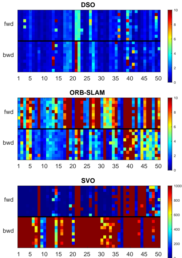
Fig. 6: Results on TUM Mono VO Dataset running forward and backward. Each method runs 10 times forward and 10 times backward on each sequence. The alignment errors e_{align} are color coded and shown as small blocks. For the first two plots we use the results obtained in [8]. Note that for the results of SVO we use a different scale on the errors.
