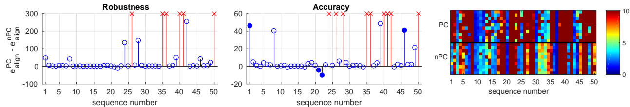
Fig. 2: Left: Performance difference of ORB-SLAM on the TUM Mono Dataset. The average of e_{align}^{PC} - e_{align}^{nPC} is shown for each sequence, where e_{align}^{PC} and e_{align}^{nPC} stand for the alignment error with and without photometric calibration, respectively. The 6 sequences on which tracking completely fails after photometric calibration are marked in red. Middle: An enlarged view of the first plot. Sequences with performance differences larger than 50 are marked in red. Solid blue dots are used to mark the 4 sequences shown in Fig. 4. Right: Color-encoded errors of all runs. Data of ORB-SLAM without photometric calibration is obtained from [10].
