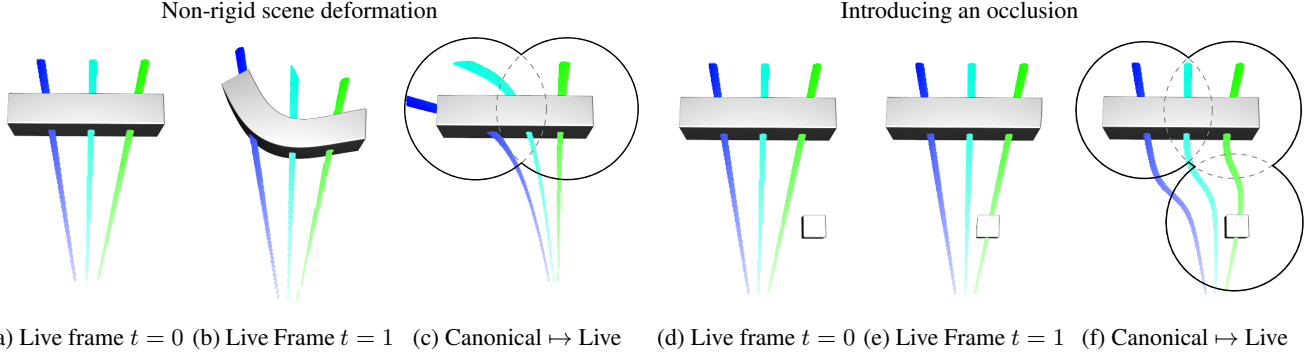
(a) Live frame t = 0 (b) Live Frame t = 1 (c) Canonical \mapsto Live (d) Live frame t = 0 (e) Live Frame t = 1 (f) Canonical \mapsto Live Figure 3: An illustration of how each point in the canonical frame maps, through a correct warp field, onto a ray in the live camera frame when observing a deforming scene. In (a) the first view of a dynamic scene is observed. In the corresponding canonical frame, the warp is initialized to the identity transform and the three rays shown in the live frame also map as straight lines in the canonical frame. As the scene deforms in the live frame (b), the warp function transforms each point from the canonical and into the corresponding live frame location, causing the corresponding rays to bend (c). Note that this warp can be achieved with two 6D deformation nodes (shown as circles), where the left node applies a clockwise twist. In (d) we show a new scene that includes a cube that is about to occlude the bar. In the live frame (e), as the cube occludes a portion of the bar, the points in the canonical frame (f) are warped to correctly pass through the cube.
