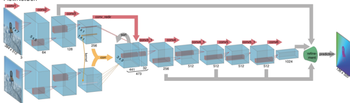
FlowNetCorr
