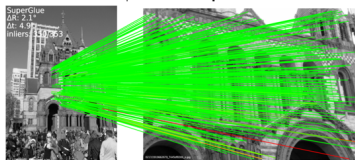
SuperPoint + SuperGlue
