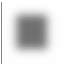
smoothed input
