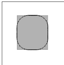
final segmentation
