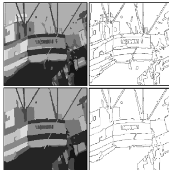
Segmentations
