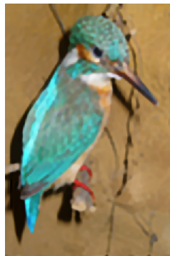
deblurred
